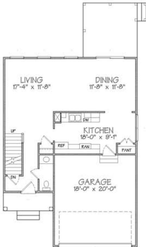
LOWER LEVEL 131 SQ FT
